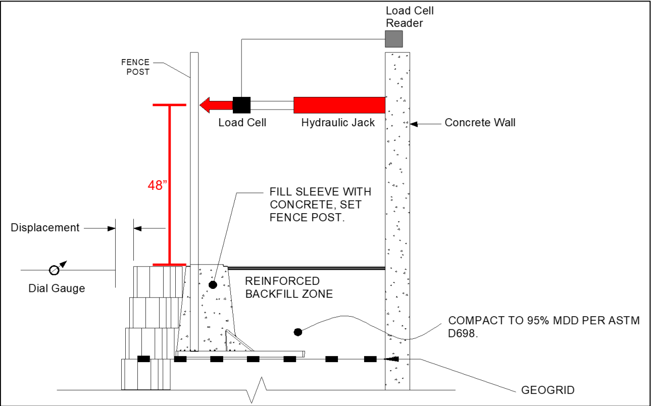
Figure No. 7: Testing Set-Up – Cardboard Tube
